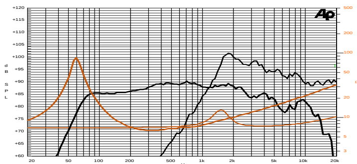
Frequency Response on 8 Lt @ 68 Hz Vented Box @ 1W, 1m Free Air Impedance
